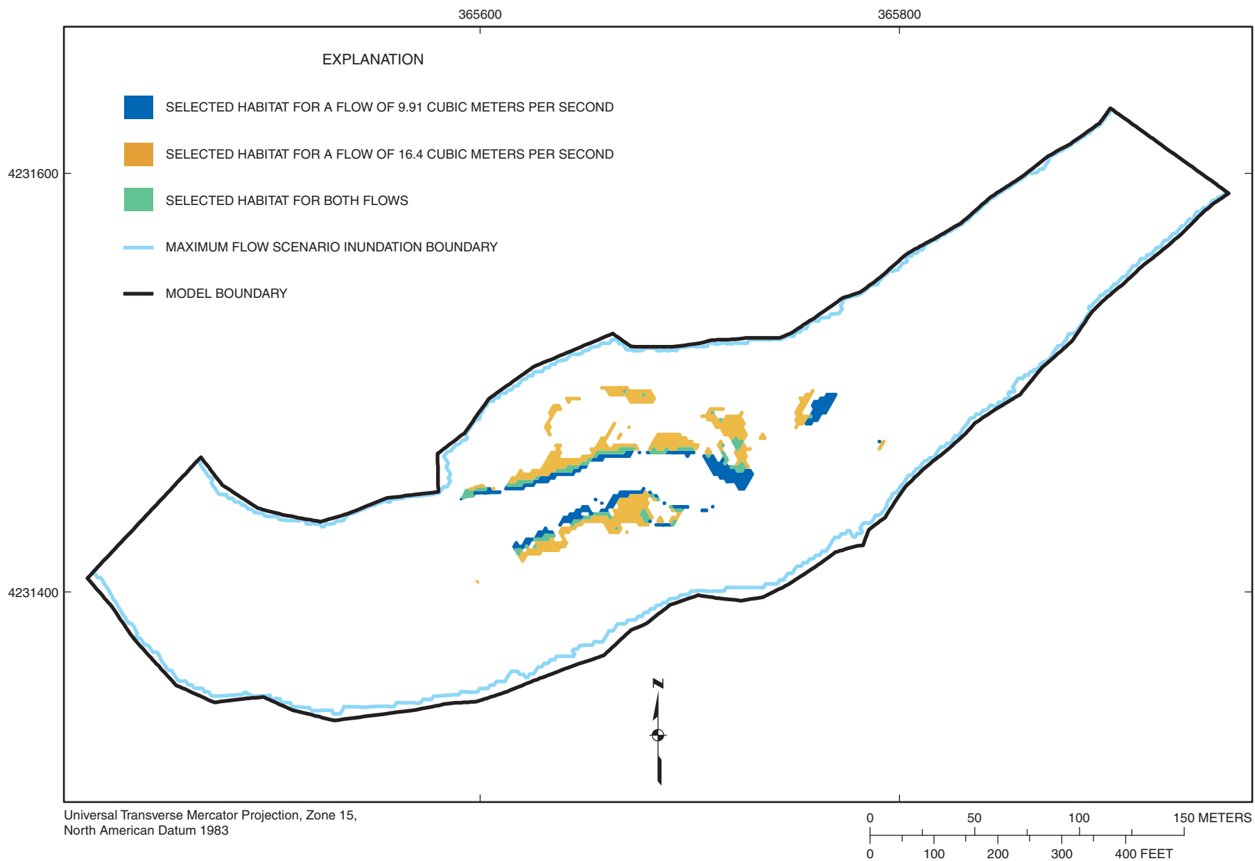
Figure 4-81. Selected habitat area distribution for habitat category 20 (flathead catfish) at flows of 9.91 and 16.4 cubic meters per second at Marais des Cygnes River site MDC2.
